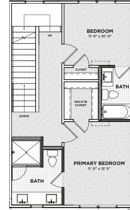
▲ FOURTH LEVEL
