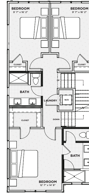
▲ THIRD LEVEL
