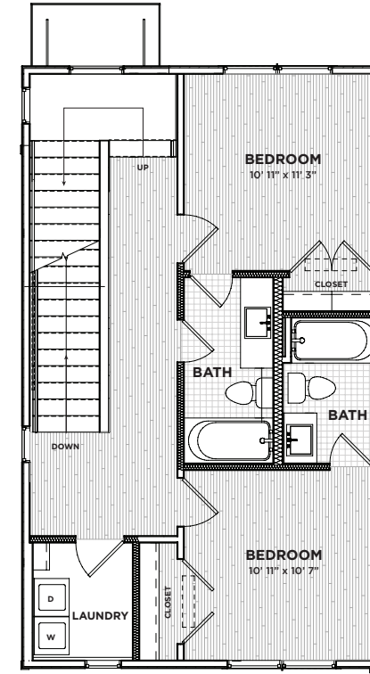
▲ THIRD LEVEL
